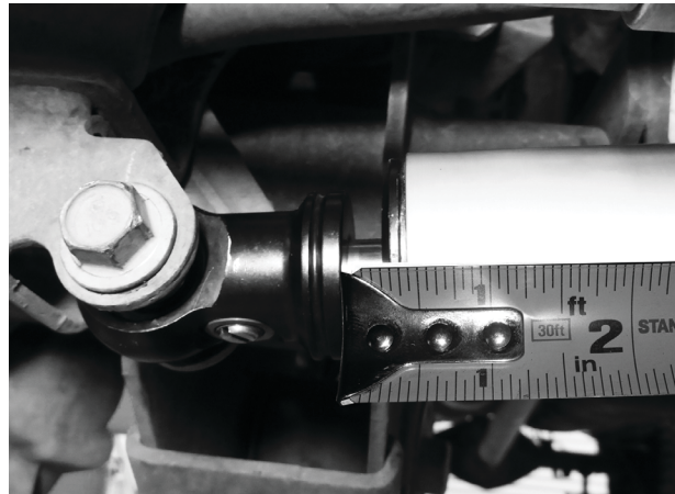
Fig. 1: Eyelet installed with 1/4" of shaft exposed.
